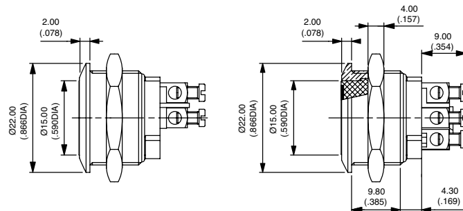
Hex nut 22 (.866) across flats
