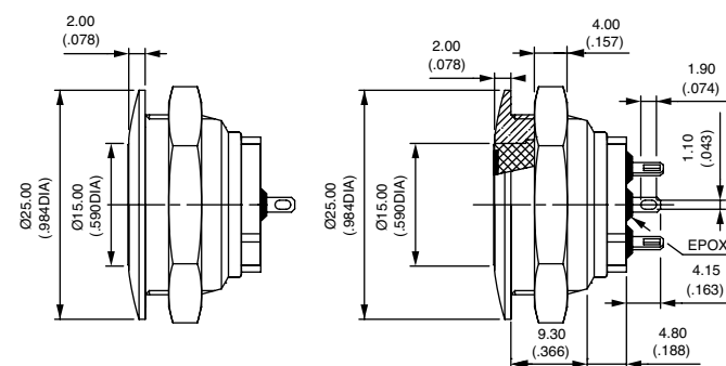
Hex nut 25 (.984) across flats
